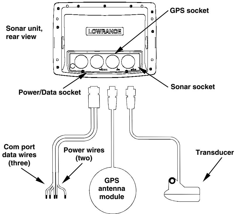
Cable connections.
