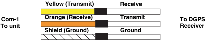
Com-1 wiring to receive DGPS position information from a DGPS receiver.
