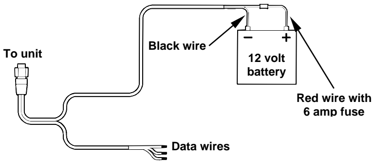
Power connections for this series sonar/GPS unit.
