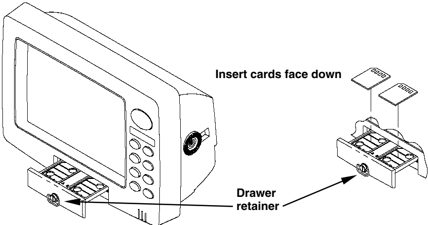
Memory card drawer on the LCX-19C and LCX-18C.
