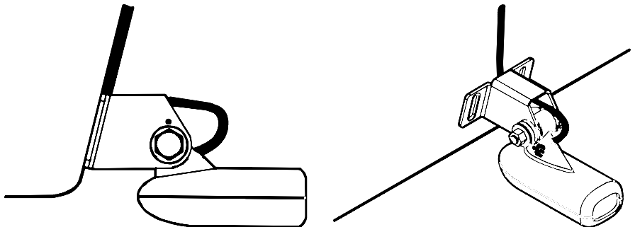
For single-frequency Skimmer, route cable over bolt and through bracket. Side view shown at left and seen from above at right.
