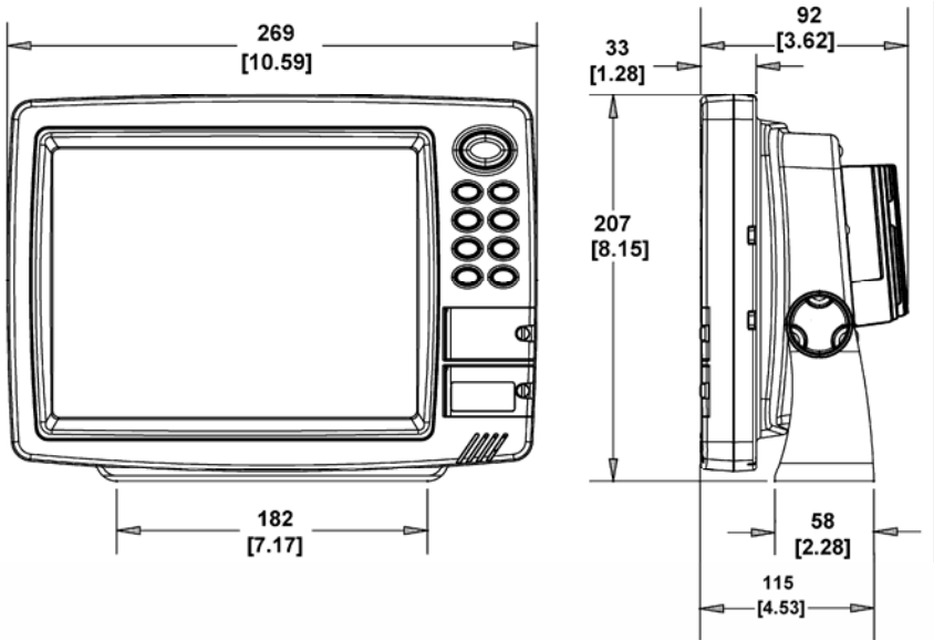
Front view (left) and side view (right) showing dimensions of the LCX-112C and LCX-113C HD mounted on gimbal brackets.
