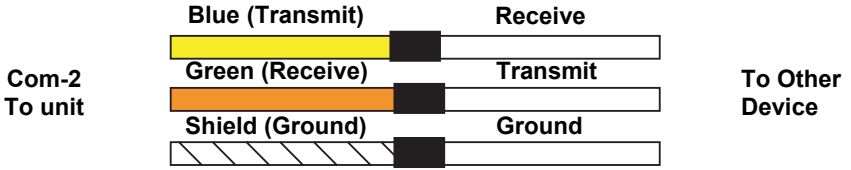
Com-2 wiring to exchange position information
