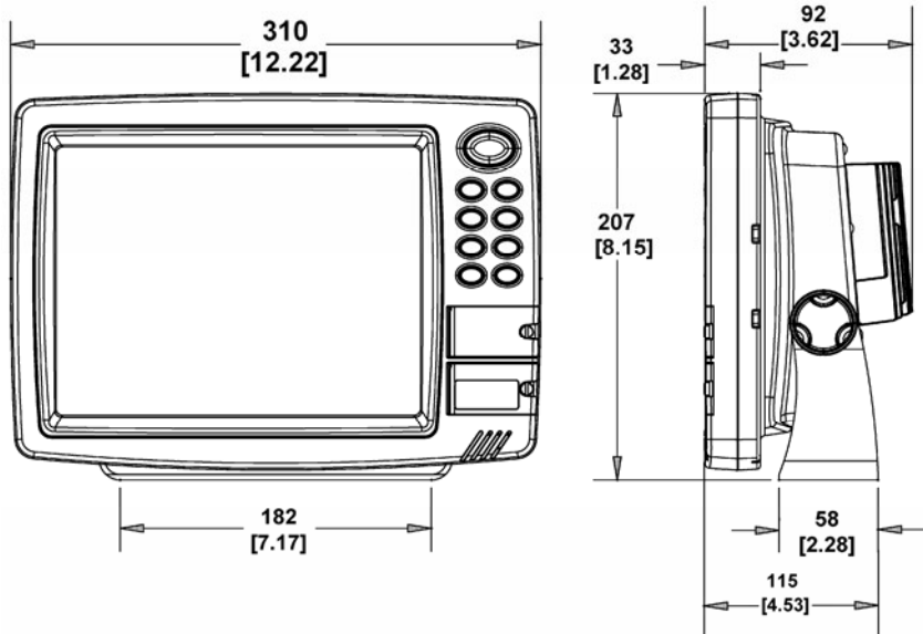
Front view (left) and side view (right) showing dimensions of the LCX-37C and LCX-38C HD mounted on gimbal brackets.
