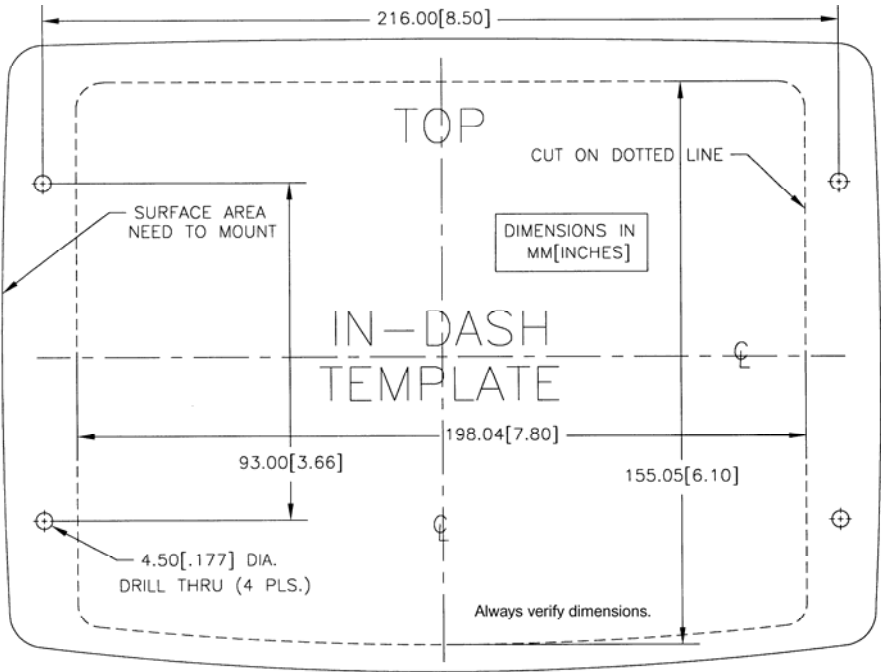
In-dash mounting template for the LCX-27C and LCX-28C HD, showing dimensions. NOTE: The figure above is not printed to scale.
