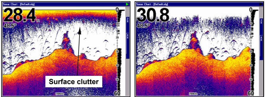
In the illustration on the left, Surface Clarity is turned off. The view on the right shows Surface Clarity set on high.
