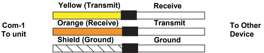
Com-1 wiring to exchange position information with another device.
